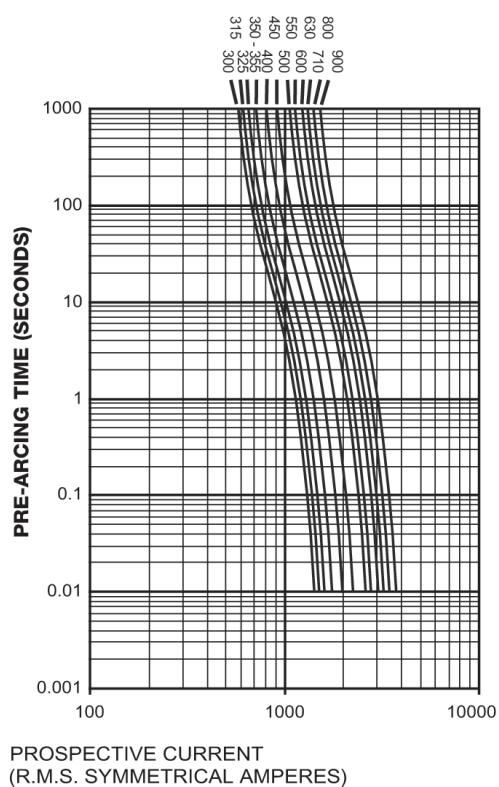
Caratter. tempo-corrente 3LS - Time-current characteristics 3LS
